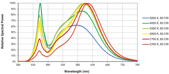
Spectral Radiant Flux VS Wavelength
